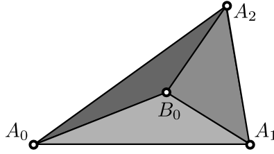
Figure 3: Illustration for the proof of Lemma 3.4
