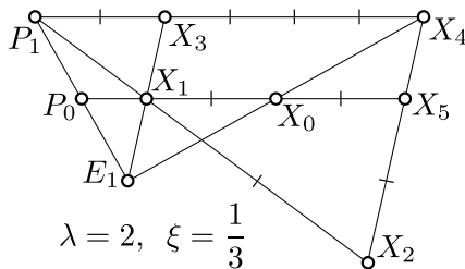
Figure 5: An illustration of Lemma 3.9
